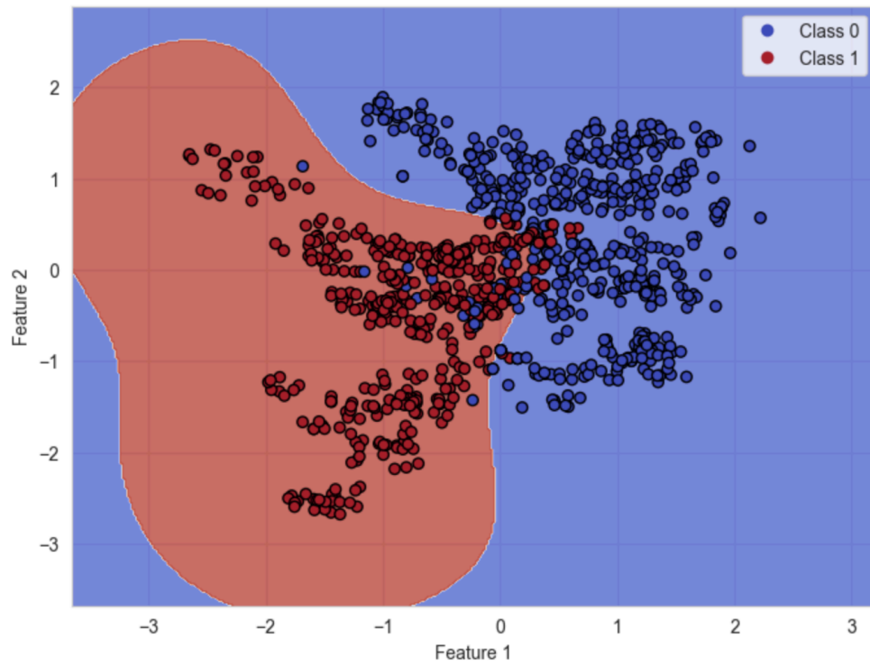
Banknote Dataset - SVM with RBF Kernel <PES2UG23CS333>
